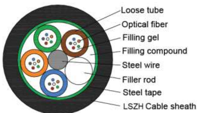
CABLE STRUCTURE AND PARAMETERS:
